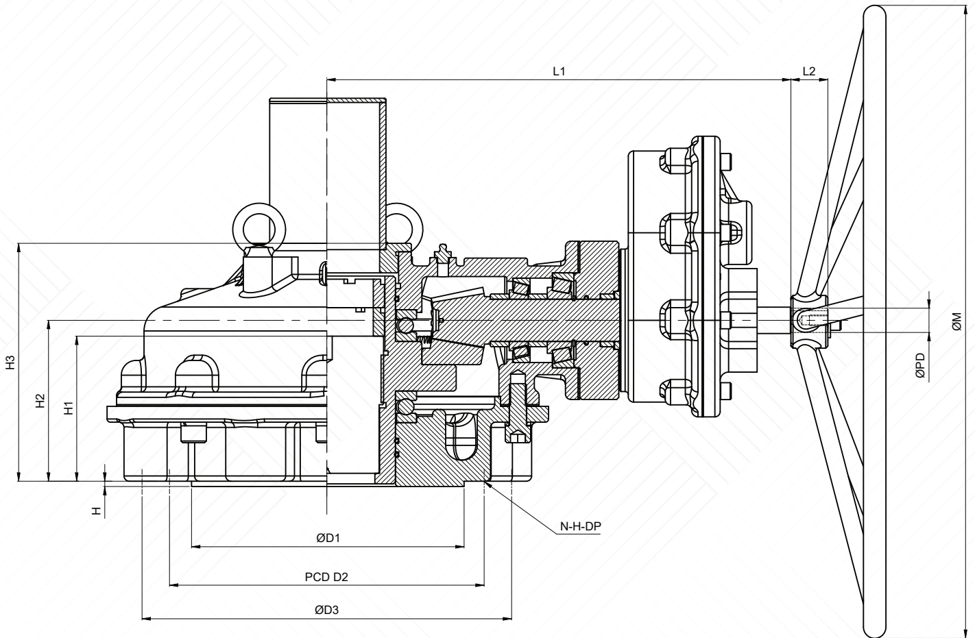
ISO 5210 Flange Mounting Details
