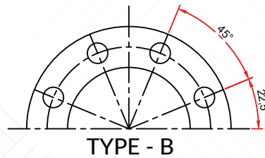
ISO 5210 Flange Mounting Details
