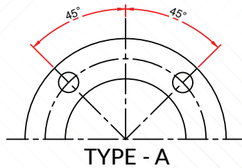
ISO 5210 Flange Mounting Details
